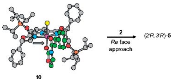
Figure 2. Assumed reacting intermediate 10 in the DA reaction between 2 and 3 , catalysed by the \text{Sc}(\text{OTf})_3 complex of pybox ( 1 ); the yellow sphere represents a triflate ligand.
