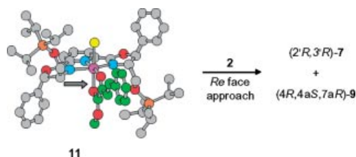
Figure 3. Assumed reacting intermediate 11 in the DA and HDA reactions between 2 and 4 , catalysed by the \text{Sc}(\text{OTf})_3 complex of pybox ( 1 ); the yellow sphere represents a triflate anion.
