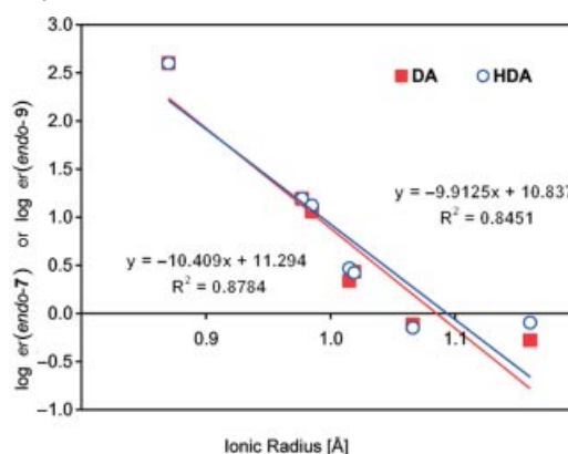
Figure 1. Plot of log er for the DA ( endo-7 ) and HDA ( endo-9 ) processes versus the lanthanide ionic radius.
